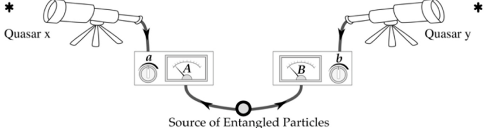
Schematic of our proposed "Cosmic Bell" experiment. A source sends entangled particles to two distant detectors. While the particles are in flight, light from distant quasars x and y is used to randomly choose the detector settings a and b on each side, which then measure experimental outcomes A and B. Many runs would be compared to confirm that the results always violate the Bell inequalities and are independent of the choices of which quasars to observe. Source: Gallicchio, Friedman, & Kaiser 2014
