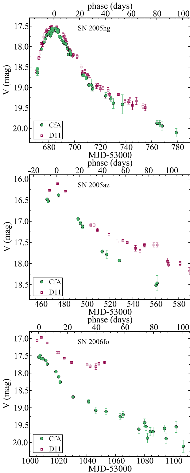
Figure 8. V -band light curves from our survey and D11 for SN 2005hg (top), SN 2005az (middle), and SN 2006fo (bottom), respectively, from the “gold,” “silver,” and “bronze” D11 subsamples (see the text). SN 2005hg shows excellent agreement in V (although an offset is present in R ), while both SN 2005az and SN 2006fo show a significant photometric offset, with D11 brighter at all epochs, a behavior observed in the majority of the objects in common between the two samples. The discrepancy grows at later epochs when the SN is fainter, which is consistent with the D11 photometry being brighter due to host-galaxy contamination in the photometric measurements. Only V -band data are shown, as the V standardized magnitudes are reported by both surveys in the same photometric system, but similar discrepancies are seen in R after photometric transformations are applied.
