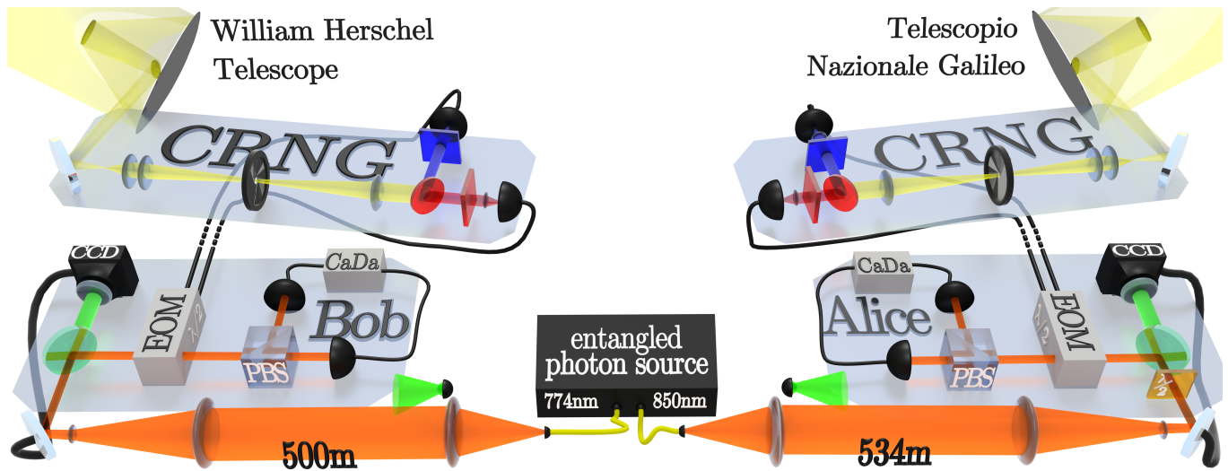
FIG. 2. A photon pair source located in the middle produced polarization-entangled photons at center wavelengths of 773.6 nm and 850 nm. The photons were separated into two spatial modes via a dichroic mirror and sent via free-space channels to the quantum receivers at Bob (773.6 nm) and Alice (850 nm). Fast steering mirrors guided the photons to the receivers using a green LED as a reference. Electro-optical modulators (EOM) rotate the measurement basis according to the input signals from the CRNGs. Polarization measurements are performed using a polarizing beam splitter (PBS) with avalanche photodiodes in each output path. Detection events are timestamped by the control and data acquisition unit (CaDa) and stored locally. Quasar light is collected by the astronomical telescopes and fed into an optical system that creates a magnified image with an iris to restrict the field of view. The quasar light is then split according to its wavelength into a “blue” and a “red” channel, whereby each channel contains additional filters to remove misdirected photons. The detector signals are used to trigger the implementation of the corresponding measurement basis at the EOM.
