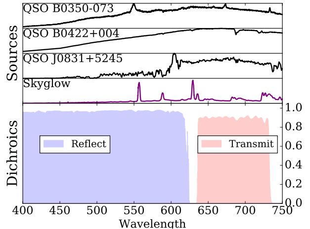
FIG. 7. Top: The number distribution of photons from each source, weighted by the transmission of optical elements and the detector efficiency. The quasar spectra are redshifted by Rayleigh scattering. Bottom: Our system of four dichroic elements splits incoming photons cleanly into a reflect (blue) channel and a transmit (red) channel. The red channel is shortpassed to reject a large fraction of Meinel rovibrational emissions which grow rapidly at wavelengths longer than \sim 700 nm. Quasar spectra were taken from: QSO J0831+5245 [79], QSO B0350-073 (SDSS DR14, [52]), and QSO B0422+004 [80]. The skyglow spectrum is from Ref. [72].
